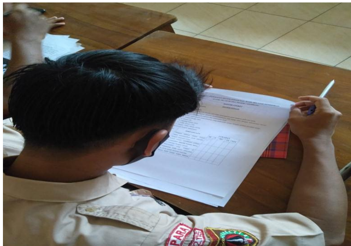
Gambar.2 Pengisian Angket
