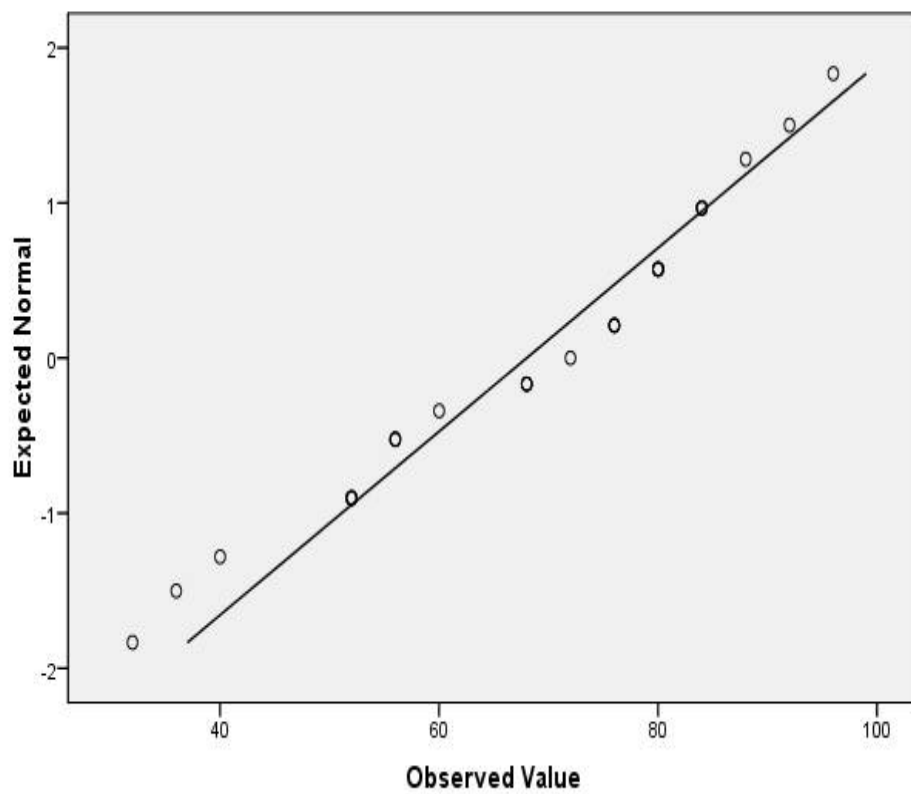
Normal Q-Q Plot of Pre Test
