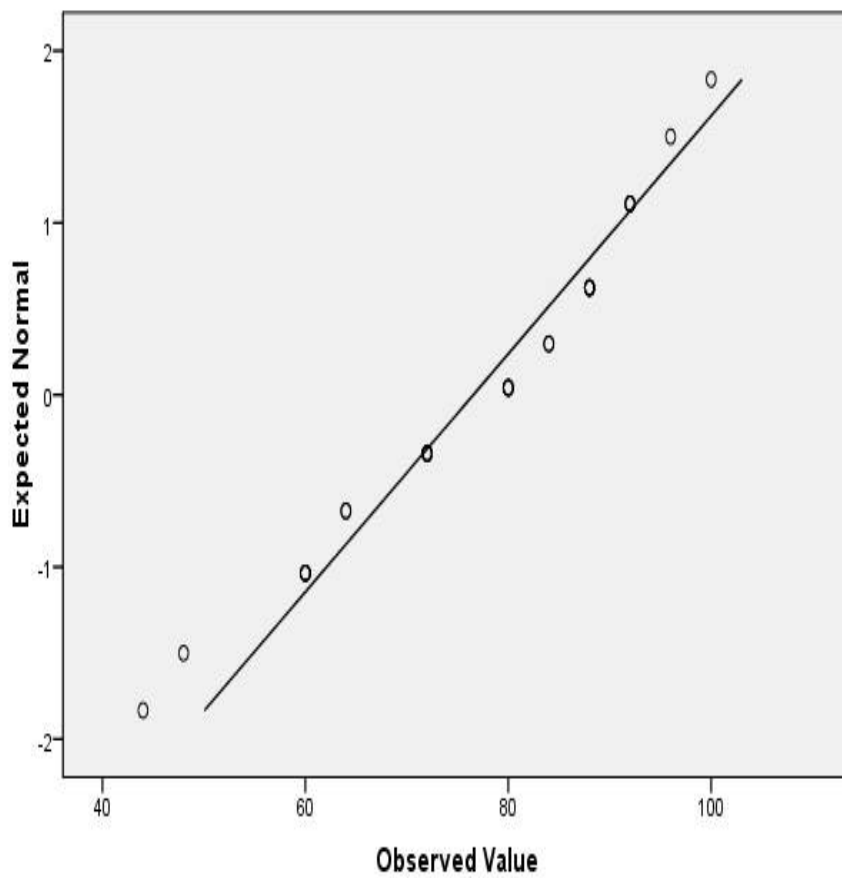
Normal Q-Q Plot of Post Test
